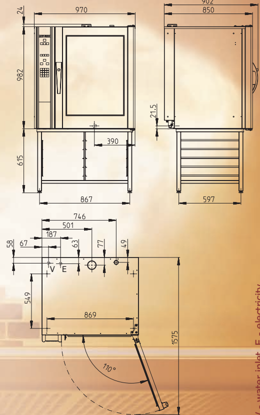
RETIGO HP 8
