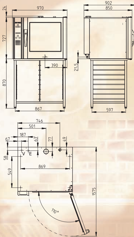
RETIGO HP 5
